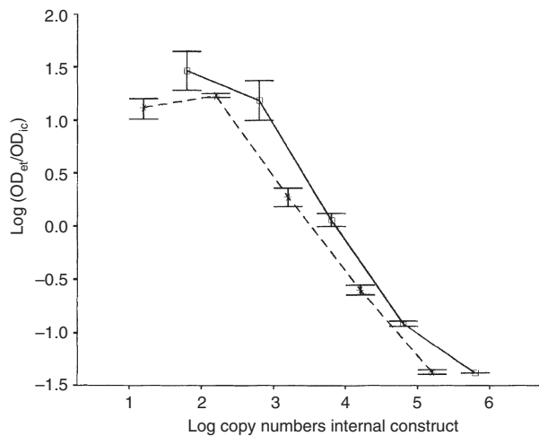
Figure 3 Analysis of HPV 16 and \beta -globin PCR-EIA. The ratio of optical densities (ODs) from endogenous template to internal construct ( OD_{E1}/OD_{IC} ) is plotted on a log-scale against the concentration of the internal construct. The median values and standard deviations are shown. (—) HPV 16, slope P = -1.08 in the range of log values between -1 and +1 ; (---) \beta -globin, slope P = -0.89 in the range of log values between -1 and +1
