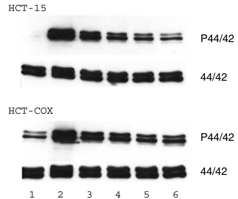
Figure 7 Phosphorylation of ERK1/2 (p42/44) after EGF stimulation in control (first two rows) and COX-2-transfected HCT-15 (third and fourth row). First lane is the control without stimulation, next lanes are 5, 10, 15, 30 and 45 min after stimulation, respectively. In rows 2 and 4, the unphosphorylated ERK1/2 (p42/44) serves as loading control. Experiments with a different cell line (HepG) gave similar results.
