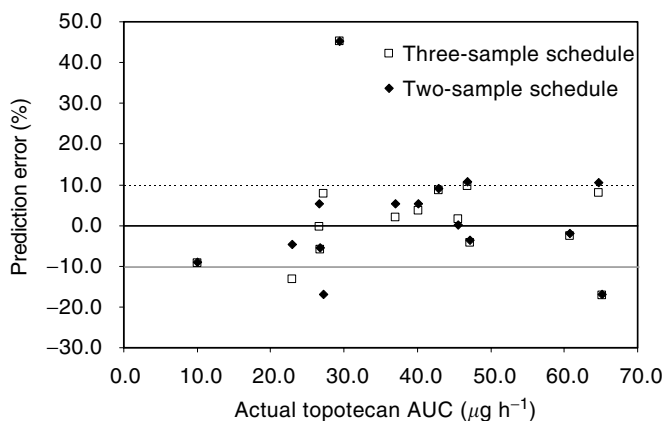
Figure 2 Ratio plot for prospective evaluation of the limited sampling applied to the oral administration of topotecan. Plasma AUC were estimated on concentrations at times 1.5 and 6 h (two-sample schedule), 1.5, 4, and 6 h (three-sample schedule) after oral administration using NONMEM.
