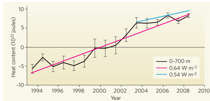
Figure 1 | Changing heat content of the global ocean, with respect to the mean of 1993 to 2008. The warming ocean is revealed by changes in heat content from 1993 to 2008, shown by the black line with error bars, as constructed by Lyman et al. 1 . This analysis samples the ocean to 700 m depth and gives an average warming trend of 0.64 \text{ W m}^{-2} (red line). The data available from Argo floats since 2003 enable an estimate to 2,000 m depth (blue line) 8 to be made. The differences between the black and blue plots after 2003 suggest that there has been significant warming below 700 m, and that rates of warming have slowed in recent years. Processing of the two data sets is not compatible, however, so firm conclusions cannot yet be drawn by comparing them.
