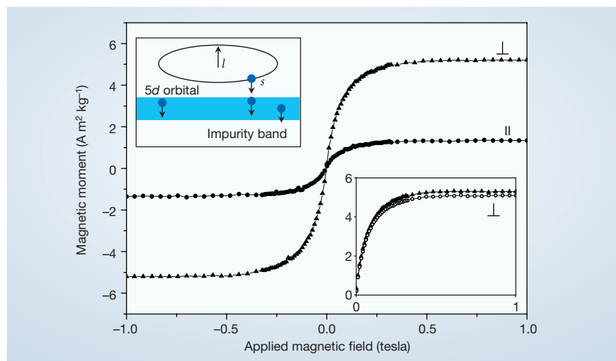
Figure 1 Magnetization curves for a thin film of hafnium dioxide measured in a superconducting quantum interference device (SQUID) magnetometer with the field parallel (||) or perpendicular (⊥) to the plane of an R-cut sapphire substrate. These room-temperature data are corrected for background diamagnetism of the substrate ( -1.8 \times 10^{-7} \text{ A m}^2 \text{ T}^{-1} ). Insets: top left, proposed coupling scheme for orbital, spin and impurity-band magnetism in hafnium dioxide (blue circles represent electrons, arrows show direction of their spin moment, the orbital and spin moments l and s of an electron in a 5 d state couple antiparallel to form a j = 3/2 state); bottom right, magnetization curves at different temperatures (triangles, 5 K; circles, 400 K).
