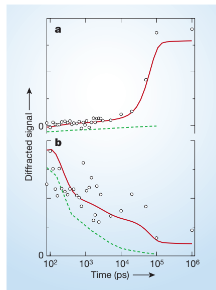
Figure 1 X-ray diffraction of iodine molecules in carbon tetrachloride solution. Plech et al. excited the iodine molecules with a laser pulse, then monitored the molecules' dissociation using X-ray pulses applied at varying time intervals after the excitation. The diffracted signal is shown here for two different spatial scales: a, 0.6 nm and b, 0.15 nm. The rise of the data in a is attributed to the solvent taking up the energy released by the iodine molecules as they relax to their ground state, and expanding. The behaviour is quite different in b: on this scale, both the relaxation of the iodine molecules and the recombination of dissociated atoms contribute to the signal. In both cases, the red curve indicates the predicted signal, taking all the relevant effects into account; the green curve represents the contribution from iodine atoms that do not escape their solvent cage.
