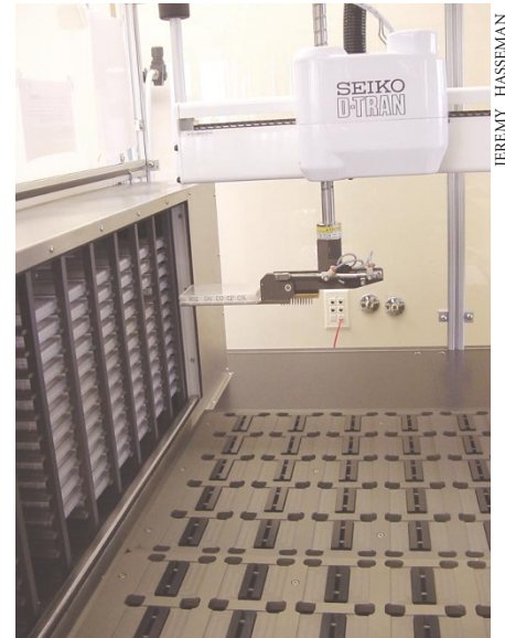
Custom-built robot arrayer in action at TIGR can spot 100 slides at a time.
