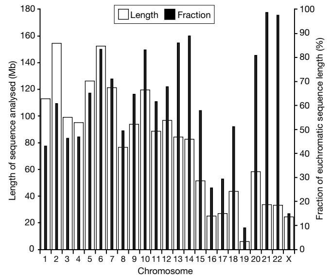
Figure 1 Sequence coverage for comparison of the genetic and physical maps. The total length of sequence used in the analysis (open bars) and the approximate percentage of the euchromatic sequence length (solid bars) are shown for each chromosome.
