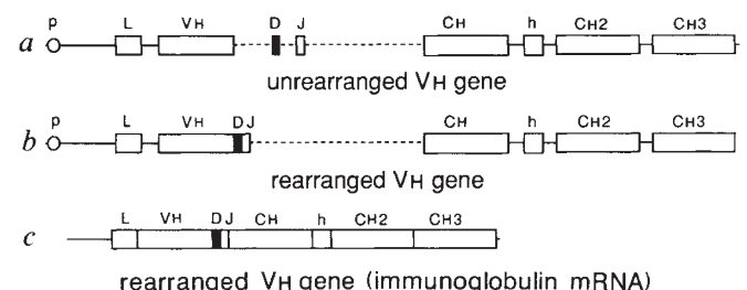
FIG. 3 Organization of V genes. The domain structure of the antibodies is mirrored at the level of the gene, as the individual domains are encoded by separate exons. In turn, the VH and VL domains are built from separate genetic elements, and assembled by DNA rearrangements during lymphocyte differentiation. Thus the first and second hypervariable loops are encoded by the germ-line V genes, but the third hypervariable loop by the combination of V, D and J elements (for the VH domain) and V and J elements (for the VL domain). The third hypervariable loop of VH is accordingly the most diverse in sequence and backbone conformation and is often the longest of the loops. Exon structure is illustrated for the unrearranged and rearranged VH genes and is similar (not shown) for VL genes (VK or VL). VH, unrearranged or rearranged heavy chain variable region as appropriate; D, D segment; J, J segment; CH1, CH2, CH3, first, second and third heavy chain constant exons, respectively; h, hinge exon; L, signal sequence; p, immunoglobulin promoter (octanucleotide motif). The potential diversity of the mouse primary repertoire is huge as a consequence of the combinatorial arrangements of the genetic elements. It can be estimated as follows. (1) Diversity due to combinatorial integration: 300 V_K \times 4 J_K = 1.2 \times 10^3 and 200 V_H \times 15 D \times 4 J = 12 \times 10^3 . (2) Diversity due to junctional alternatives (alternative readings at junction due to differences in reading frame, and lengths of J and D segments): V_K to J_K \sim 3 and V_H to D to J \sim 40 . (3) Diversity due to N segment for heavy chain > 10 . (4) Hence combined diversity for each chain: light chains = 3 \times 10^3 and heavy chains > 5 \times 10^6 . Conclusion: diversity due to combinatorial association of heavy and light chains > 10^{10} . Additional factor due to somatic mutation > 10^{30} (see text).
