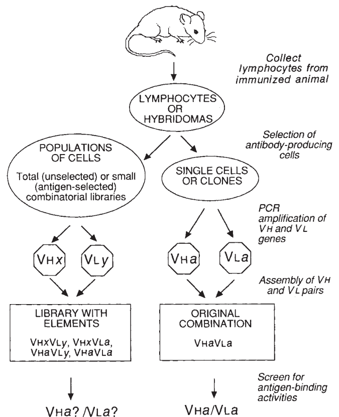
FIG. 5 Strategies for cloning paired VH and VL genes from lymphocytes of an immunized animal. VH and VL genes (expressed as pairs VHx/VLy) from n lymphocytes can be amplified by PCR from the mRNA or genomic DNA of single cells or populations. The lymphocytes can also be selected by antigen-binding, or immortalized as hybridomas by fusion with myeloma cells or by infection with Epstein-Barr virus. From single lymphocytes, or clones, the original VHa/VLa gene combination is readily rescued. From populations of lymphocytes, repertoires of VH-VL genes (VL n ) could be combined at random, and antigen-binding combinations selected. But for large populations of lymphocytes, original combinations of VH and VL genes will be a minor proportion of heterologous combinations, some of which may display residual antigen-binding activity. The library will contain (n-1)^2 VHxVLy elements, (n-1) each of VHxVL a and VHaVLy elements and a single VHaVL a element. VHa and VLa (or close derivatives), however, may occur repeatedly. Thus, at earlier stages or immunization, there are likely to be some artificial pairs which originate from different but closely related clones which can bind antigen, particularly with responses dominated by 'unique' VH and VL gene combinations (restricted or idiotypic responses 59,60 ). Ref. 90 is in agreement with this prediction. As maturation for high affinity proceeds, the number of mutations increase and the likelihood of effective heterologous complementation diminishes.
