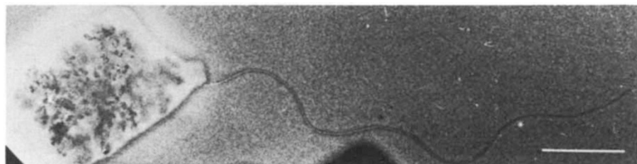
Electron micrograph of a square bacterium with a single flagellum negatively stained with phosphotungstic acid. The bar indicates 1 \mu m. From Alam, M. et al. EMBO J. 3 , 2899; 1984.
