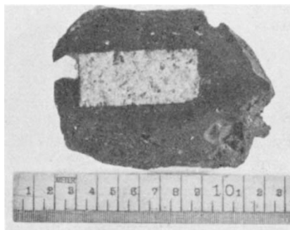
Fig. 1 Perfectly rectangular block of ultramafic xenolith in alkalic lava from the Mt Schank volcano in SE Victoria, Australia. (Photograph courtesy of Dr Alan Moore, University of Cape Town, South Africa.)
