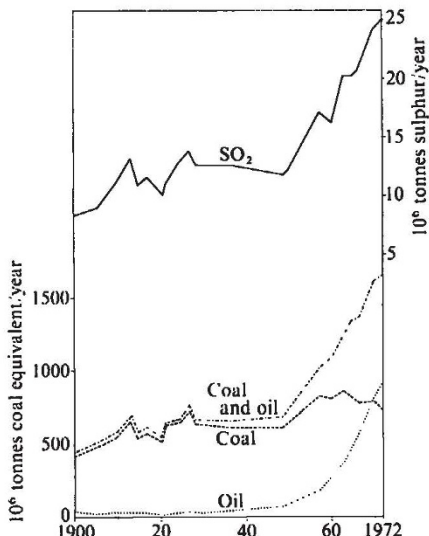
Fig. 1 Fossil fuel consumption and estimated anthropogenic SO 2 emissions in Europe 1900–1972 (Source: After Fjeld Nilu Teknisk Notetnu 1/76 (1976)).
