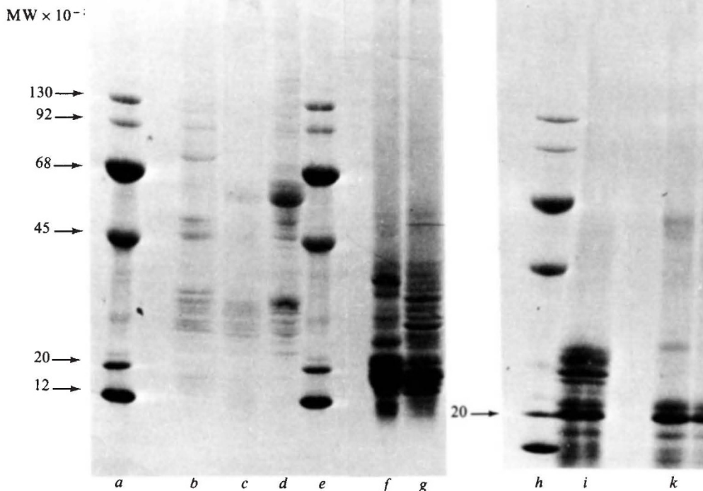
Fig. 4 Analysis of proteins present in purified polysomal and informosomal mRNP particles from rabbit reticulocytes. mRNP particles were dissolved in SDS-sample buffer, boiled and loaded on to a 7–18% polyacrylamide gradient gel containing SDS 15 . Channels a, e, h , marker proteins: \beta -galactosidase (MW 130,000), phosphorylase b (92,000), bovine serum albumin (68,000), ovalbumin (45,000), \alpha_2 -crystallin (20,000), cytochrome c (12,000). b , Polysomal 15S mRNP. c , Informosomal mRNP after a 0.5 M KCl wash (see also i ). d , Informosomal mRNP before the 0.5 M KCl wash. f , EDTA-treated 40S ribosomal subunits. g , EDTA-treated 60S ribosomal subunits. l , Informosomal mRNP after a 0.5 M KCl wash (double band at 20,000 is carrier \alpha -crystallin). k , 0.5 M KCl wash of informosomal mRNP (double band at 20,000 carrier is \alpha -crystallin).
