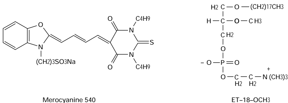
Figure 1 Structures of MC540 and ET-18-OCH 3 .
