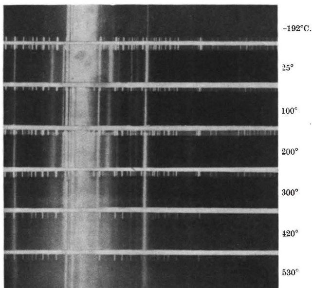
LIGHT SCATTERING IN QUARTZ.
