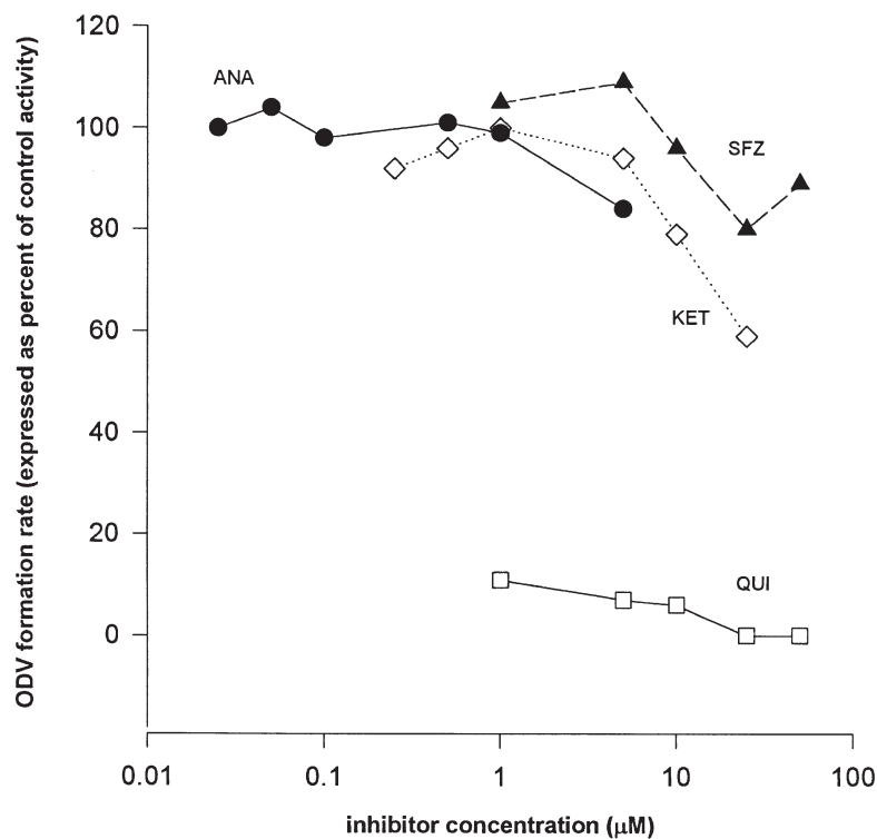
Figure 3. Effect of varying concentrations of ketoconazole ( \diamond ), quinidine ( \square ), sulfipyrazone ( \blacktriangle ), and \alpha -naphthoflavone ( \bullet ) on the formation of O-desmethylvenlafaxine. Each point is the ratio, expressed in percent, of the reaction velocity at the indicated inhibitor concentration divided by the velocity with no inhibitor.
