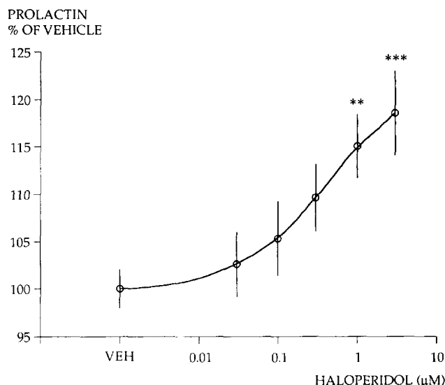
Figure 1. Effect of various concentrations of haloperidol (30 nM, 100 nM, 300 nM, 1 \mu M, 3 \mu M) on prolactin release from GH 4 C 1 -hD 2 s cells. The curve was analyzed using UltraFit (BioSoft, Ferguson, MO, USA); goodness of fit (logistic sigmoid) was 0.97; EC 50 was 425 nM, n = 28 . Stars indicate level of significance versus vehicle: ** p < .01 , *** p < .001 (ANOVA followed by Fisher's PLSD test).
