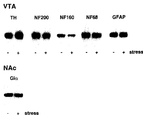
Figure 1. Autoradiograms showing the effect of chronic unpredictable stress on levels of TH, NF, and GFAP immunoreactivity in the VTA and on levels of G \alpha immunoreactivity in the NAc of Sprague-Dawley rats. VTA or NAc extracts from control and chronic (10 days) stress-treated rats were subjected to one-dimensional SDS-polyacrylamide gel electrophoresis, to blot immunolabeling for TH, NF-200, NF-160, NF-68, GFAP, or G \alpha , and to autoradiography as described in Methods.
