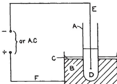
FIG. 1. Diagram of apparatus for preparation of colloidal metals: A , cellulose acetate cup; B , mercury bath; C and D , tricesylphosphate; E and F , metallic electrodes.
