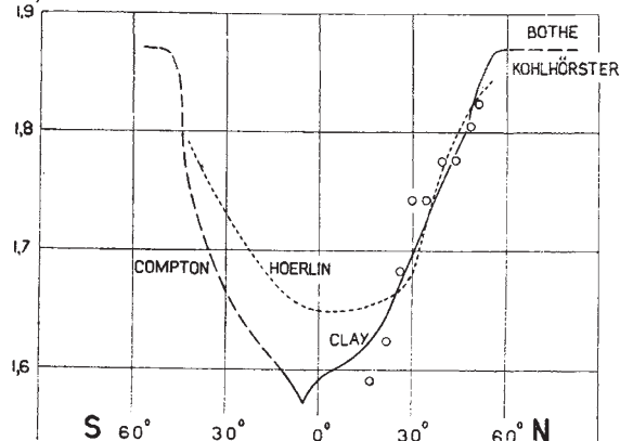
Fig. 1. Latitude effect of cosmic radiation. Circles indicate results of author. Vertical scale indicates number of pairs of ions in normal air.
