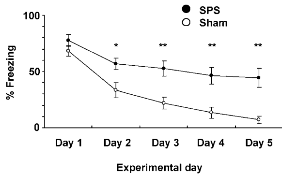
Figure 2 Influence of SPS on fear extinction. Data are expressed as mean \pm SEM of 10 rats per group. On day 1, there were no significant differences in the freezing levels between the Sham and SPS groups. However, on days 2–5, the SPS group showed impaired extinction compared to the Sham group. * p < 0.05 , ** p < 0.01 ; unpaired Student's t -test.
