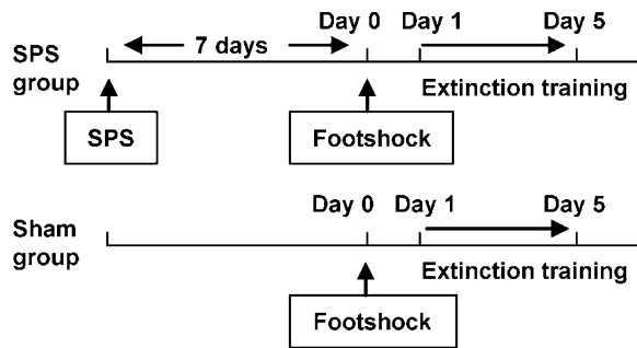
Figure 1 Treatment groups and procedure. In the SPS group, 7 days after SPS treatment, contextual fear conditioning was performed (on day 0), and then extinction training was performed on each of five consecutive days following fear conditioning. In the Sham group, the procedures were similar except that SPS treatment was not performed.
