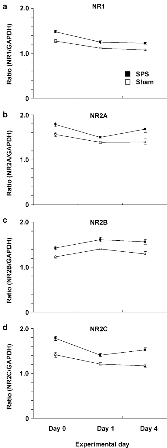
Figure 5 Comparison of the levels of NMDAR mRNAs (NR1 (a), NR2A (b), NR2B (c), NR2C (d)) across experimental timepoints. Data are expressed as the ratio of the concentration of the target molecule to that of GAPDH (target molecule/GAPDH) and represent the mean \pm SEM (day 0: Sham; N=6 , SPS; N=6 , day 1: Sham; N=7 , SPS; N=7 , day 4: Sham; N=9 , SPS; N=9 ).
