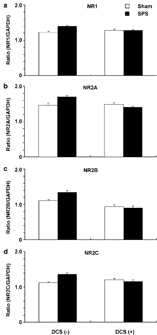
Figure 6 Effects of repeated DCS administration on the levels of NMDAR mRNAs (NR1 (a), NR2A (b), NR2B (c), NR2C (d)) on day 4. Data are expressed as the ratio of the concentration of the target molecule to that of GAPDH (target molecule/GAPDH) and represent the mean \pm SEM of nine rats per group.
