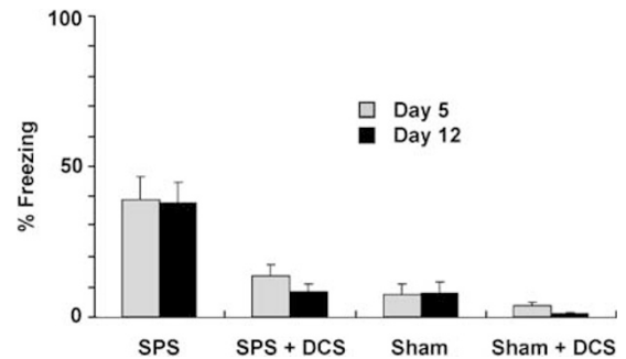
Figure 4 Effects of repeated DCS administration upon fear extinction a week after extinction training. Data are expressed as mean \pm SEM of nine rats per group.
