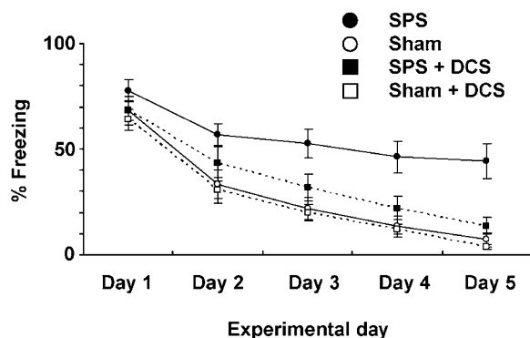
Figure 3 Effects of repeated DCS administration on fear extinction. Data are expressed as mean \pm SEM of 10 rats per group.
