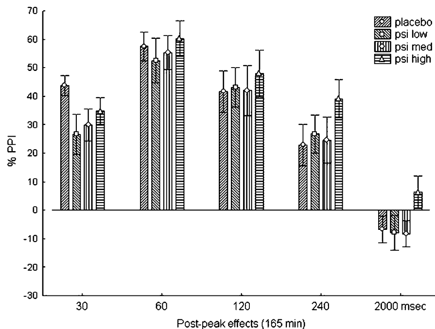
Figure 5 Dose–response effects of psilocybin on percentage prepulse inhibition (%; mean \pm SE) at five PP conditions (ISI: 30, 60, 120, 240, and 2000 ms) in healthy human volunteers during the psychological post-peak phases of the drug ( n = 16 ). ISI = interstimulus-interval.
