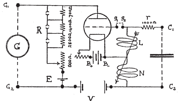
FIG. 1.—Diagram of connexions: B 1 , 4 to 6 volts; V, 30 to 100; E, 1.5 to 6. L, N, about 10 cm., flat, 150 turns. G, aperiodic galvanometer, 10 -8 amp. per div.
