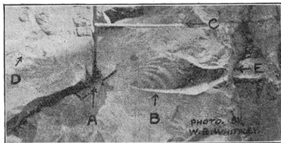
FIG. 1.—Splash-like fracture-surface due to gelignite explosion in rock. A, base of 1½" diameter drill-hole and origin of explosion; B, fluted "splash effect"; C, 2-ft. rule, to fix scale; D, one of a number of radial "splash" lines.
