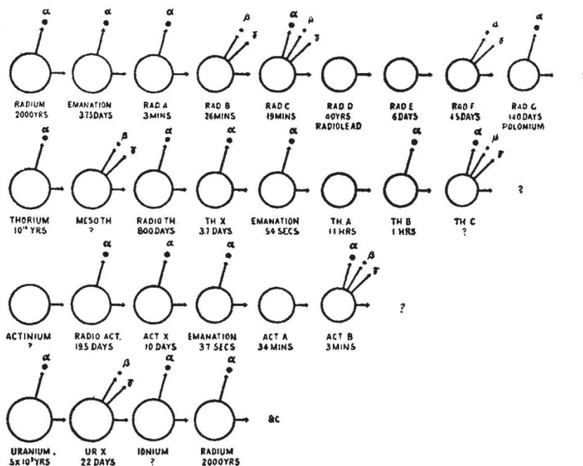
Succession of Substances produced by the transformation of radium, thorium, actinium, and uranium. The period of transformation of each substance is added below.
