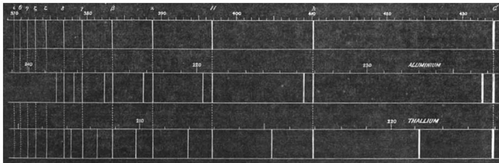
DESCRIPTION OF THE DIAGRAM - The graduations define the lines according to their wave-lengths. The first line represents the dark lines of the violet and ultra-violet spectra of the white stars. The second represents a double series of inverted lines in the ultra-violet spectrum of aluminium (electric arc). The scale of the drawing has been chosen in a manner to make G and \delta coincide with the homologous lines of the first series (first line of each doublet). One could have operated in the same way with the second series (second lines). This mode of representation advantageously replaces the numerical tables, showing the verification of the two empiric formulas—
