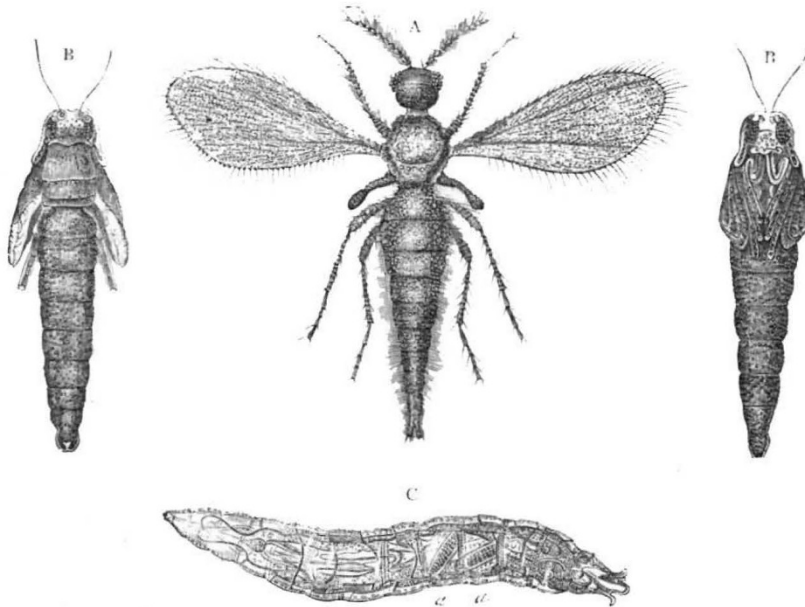
FIG. 1.—Cecidomyiid with viviparous larva. A, adult insect; B, pupa; C, larva, showing young larvæ at a a .
