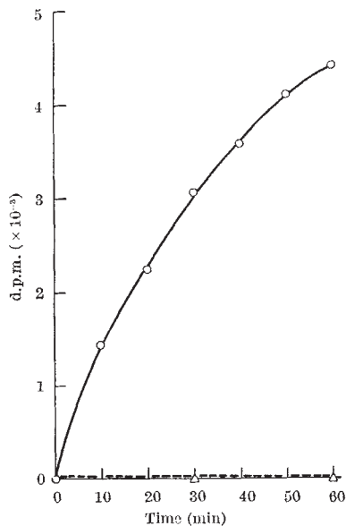
Fig. 1. Kinetics of incorporation. Virus treated with 'Nonidet' and dithiothreitol at 0° C and incubated at 37° C (○—○) or 80° C (△ --- △) for 10 min was assayed in a standard polymerase assay. ○, Unheated; △, heated.
