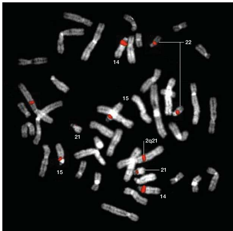
Figure 3 | In silico versus cytogenetic analysis of the human genome. In situ hybridization of a bacterial artificial chromosome (BAC) probe (RP11-140M6), which has been mapped to a highly duplicated region of 22q11 (REF. 10), is shown. Multiple signals correspond to sites of duplication. Particularly strong signals are detected on 14q11, corresponding to multiple copies of this locus as confirmed by extensive sequence analysis of chromosome 14 MONOCHROMOSOMAL HYBRIDS 10 . No evidence of this duplication can be detected on the basis of the sequence analysis of the genome. Fluorescence in situ hybridization (FISH) results pinpoint potential gaps in the finished genome. Reproduced with permission from REF. 10 © University of Chicago Press (2002).
