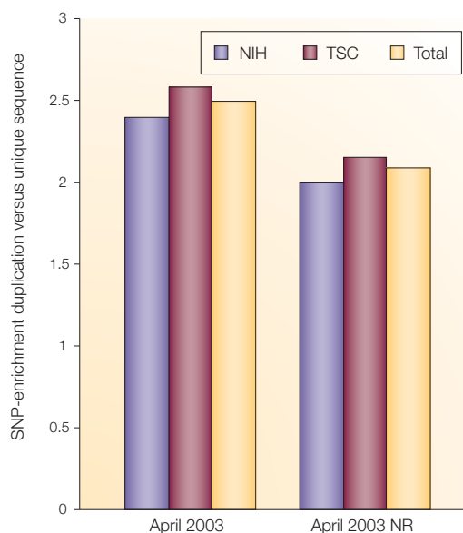
Figure 5 | SNP enrichment in duplicated sequences. SNP density between duplicated regions and unique regions was assessed in the finished genome (April 2003). 429,999 SNPs mapped to 154.0 Mb of duplicated sequence compared with 3.02 million SNPs that were assigned to 2.87 Mb of unique sequence. Based on the density of SNPs, this represents a 2.5-fold enrichment in duplicated regions of the genome. If SNPs are only allowed to be placed once in the genome (that is, multisite SNPs are counted once), this enrichment drops to 2.16-fold. SNP data are categorized on the basis of source (NIH or TSC). NIH, National Institutes of Health; NR, non-redundant; TSC, The SNP Consortium).
