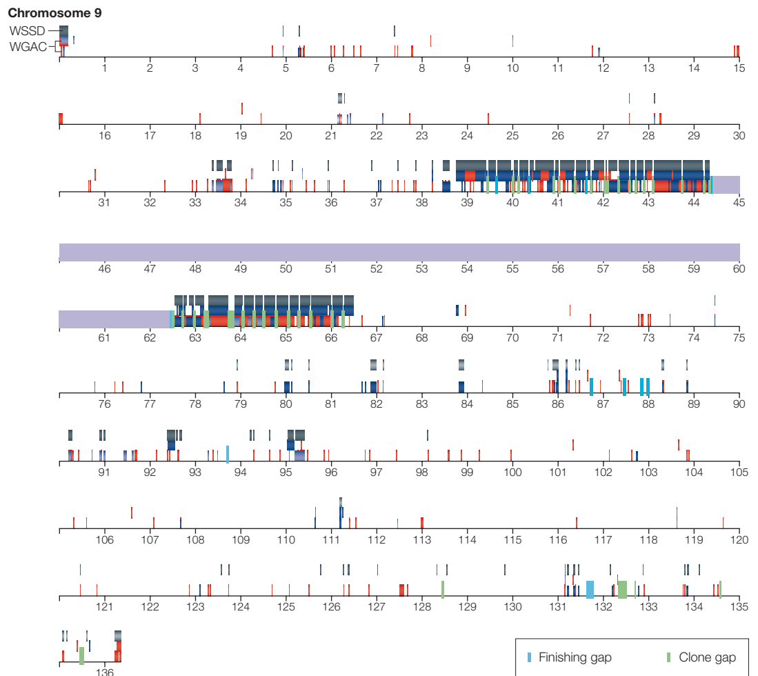
Figure 2 | Duplications and sequence gaps. Duplication content for chromosome 9 is shown as coloured (red and blue) or dark grey bars above the horizontal line (determined by WGAC and WSSD methods, respectively). The position of euchromatin sequence gaps is shown as light blue (finishing gaps) or light green vertical bars (clone gaps) that traverse the horizontal line. Centromeric satellite sequences are depicted in purple. Most (90%) of the sequence gaps associate with segmental duplications. WGAC, whole-genome analysis comparison; WSSD, whole-genome shotgun sequence detection.
