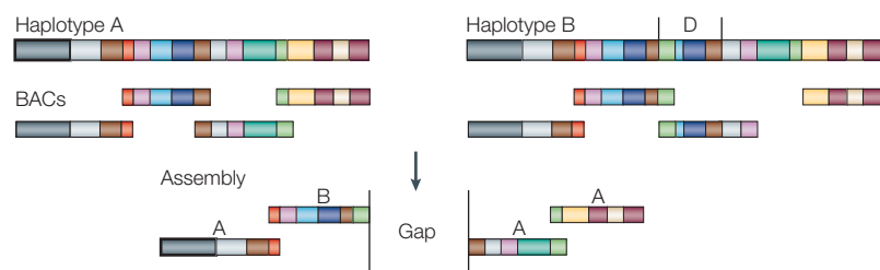
Figure 4 | Gaps, duplications and structural variation. A hypothetical large-scale structural variant (D) is shown in a highly duplicated region (duplicated segments are shown as coloured bars). Sequencing of targeted bacterial artificial chromosomes (BACs) from a diploid source leads to inconsistencies when assembly is attempted from both haplotypes (A and B). Sequence-assembly overlap from both haplotypes creates a de facto gap (green). It is impossible to assemble this region unless single haplotype continuity is obtained.
