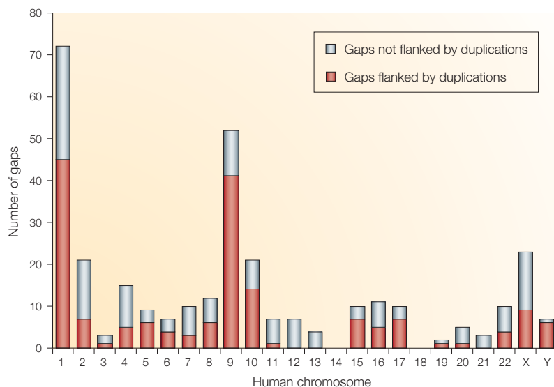
Figure 1 | Chromosomal distribution of sequence gaps. The number of euchromatic sequence gaps that are flanked by segmental duplications and by unique sequence are shown per chromosome. A total of 321 sequence gaps of the 379 gaps were classified as interstitial euchromatin. Although euchromatic and heterochromatic DNA cannot be simply defined at the sequence level, for the purpose of this analysis we considered pericentromeric DNA (distal to the most proximal block of satellite DNA) as euchromatic, because there is evidence of transcription in these regions. We did not consider the 58 gaps that are largely repetitive and for which there is little evidence of transcription (including telomeric ends, acrocentric portions or centromeric (primary or secondary constriction) satellites of human chromosomes).
