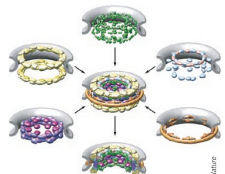
An integrated structural model for the nuclear pore complex.
