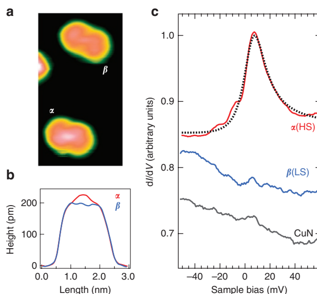
Figure 3 | SCO Fe-phen molecules on CuN/Cu(100). (a) STM image ( 3 \times 5.5 \text{ nm}^2 ) of isolated Fe-phen molecules on the CuN/Cu(100) surface with two conformations denoted as \alpha (HS) and \beta (LS) and (b) line scans across the long axis of the molecules showing the difference in their appearance. (c) dI/dV spectra taken on the centre of the two configurations of the Fe-phen molecules together with a Fano fit (dotted black line) to the Kondo resonance of type \alpha . The black line is the spectrum recorded on bare CuN with the same tip.
