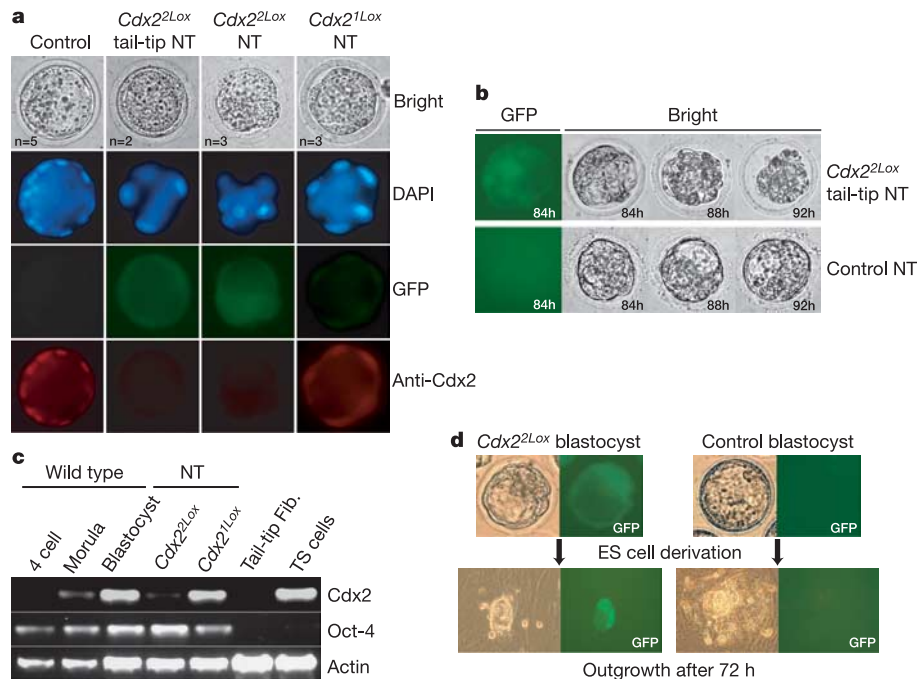
Figure 2 | Cdx2 -deficient blastocysts and ES cell derivation. a , Cdx2 immunostaining of day 3.5–4.5 wild-type and nuclear transfer blastocysts. The following donor cells were used for the nuclear transfer (from second column, left to right): Cdx2 2Lox tail-tip, Cdx2 2Lox ES cells, and Cdx2 1Lox ES cells. b , A typical Cdx2 2Lox tail-tip nuclear transfer blastocyst is shown 84 h after activation of the reconstructed oocytes. Cdx2 -deficient blastocysts initially cavitated but failed to maintain the blastocoel and collapsed. Below, an expanded nuclear transfer blastocyst derived from control cells is shown. c , RT-PCR analysis of normal and Cdx2 -deficient nuclear transfer pre-implantation morula/blastocysts. Four 4-cell embryos were pooled and RNA
