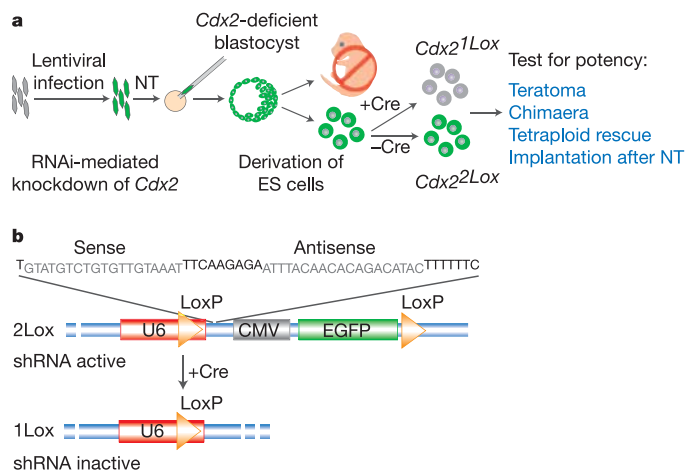
Figure 1 | Derivation of NT-ESCs from Cdx2 -deficient blastocysts.
