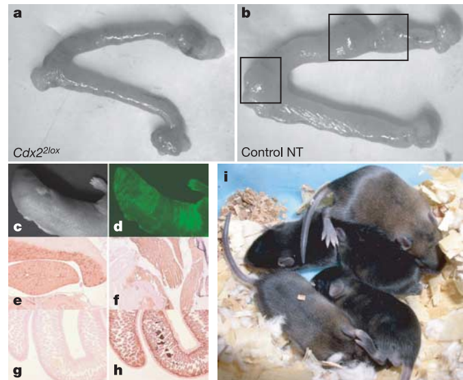
Figure 3 | Cdx2 -deficient cells maintain developmental potential but are unable to implant after nuclear transfer. a, b , In each example shown, five nuclear transfer blastocysts were transferred at day 3.5 into the uterus of a day 2.5 pseudo-pregnant female. a , Cdx2 -deficient blastocysts fail to implant. A representative uterus isolated at day 6.5 is shown. No decidua were detectable from transplanted Cdx2 -deficient blastocysts. b , Control nuclear transfer blastocysts showed normal implantation sites at day 6.5. c , Bright-field image of a postnatal Cdx2 2Lox ES chimaera. d , GFP signal indicates a contribution from Cdx2 2Lox ES cells. e-g , Histological sections and anti-GFP staining from a newborn Cdx2 2Lox chimaera. There was a contribution to the liver (endoderm; e ) and muscle (mesoderm; f ) but not to the intestine ( g ). h , Anti- Cdx2 staining of the intestine shown in g . i , Coat colour contribution of Cdx2 2Lox ES cells. Recipient blastocysts have a C57BL/6 × DBA/2 F 1 background and the Cdx2 2Lox ES cells a C57BL/6 × 129SvJae background. The presence of agouti (129/SvJae) fur indicates donor cell contribution. A litter with one wild type (black mouse below the top agouti), two low-contribution (middle) and two high-contribution chimaeras are shown.
