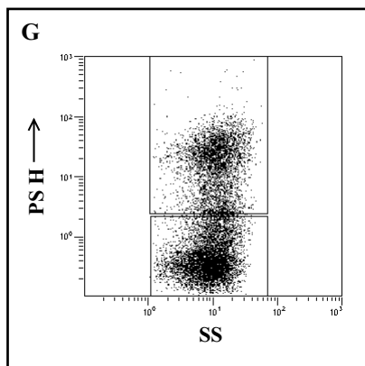
Web Fig 2. Flow cytometric analyses demonstrating variable expression (ON-OFF) of B: PS C, C: PS D, D: PS E, E: PS F, F: PS G, G: PS H. All primary antibodies were derived in rabbits and were monospecific for the indicated polysaccharide. Secondary antibody was a phycoerythrin-labeled anti-rabbit IgG. Panel A indicates an unlabeled population.
