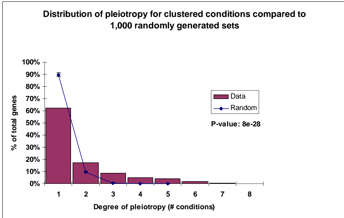
Supplementary Figure 6. Distribution of pleiotropy for clustered conditions from Supplemental Figure 5, compared to 1,000 randomly generated sets. These distributions are significantly different as assessed by the Kolmogorov-Smirnov test with a p-value of 8 \times 10^{-28} .
