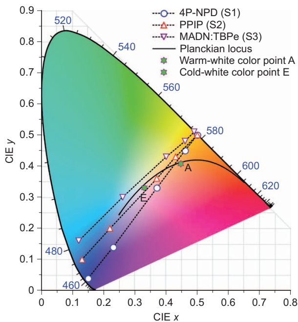
Figure 4 Color coordinates corresponding to the emission spectra presented in Figure 3 for S1, S2 and S3.
