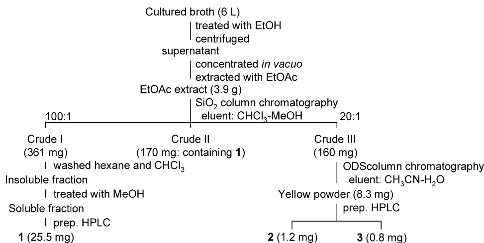
Fig. 3 Purification procedures of fungierin and hydroxyfungierins from the culture broth of Metarhizium sp. FKI-1079.
