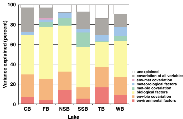
Figure 5 Results of bacterioplankton variance partitioning for each lake. Variance in bacterial community composition over time (assessed by ARISA relative fluorescence) was partitioned among meteorological (met), environmental (env) and biological (bio) sets of variables using partial canonical correspondence analyses. The sets of potential explanatory variables were defined as follows: environmental – pH, total P, total N, DOC and water temperature; meteorological – 3-day moving average of mean daily air temperature, PAR and precipitation; biological – chl a, phytoplankton populations and HNF were used as biotic explanatory variables for the bacterioplankton data set, cladoceran zooplankton populations were used as biotic explanatory variables for the phytoplankton data set. The suite of biotic variables explains much of the variance in bacterial community composition over time in each lake. See Figure 1 legend for lake acronym definitions.
