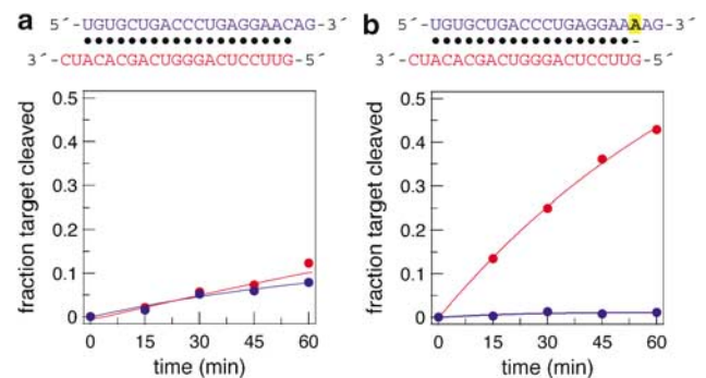
Figure 2 Use of rules of siRNA asymmetry for RNAi of huntingtin mRNA. Incorporation of the guide strand into RISC determines the RNAi activity of a siRNA. In the experiment shown here, the blue strand is the passenger in the siRNA and the red strand is the guide. (a and b) The ability of the guide strand (in red) to effect RNAi is tested against a synthetic huntingtin mRNA target (in red in figure). The RNAi activity of the passenger strand (in blue) is tested against an artificial mRNA target to which it has complementarity (in blue in figure). (a) Both the guide strand and the passenger strand have equal potency in cleaving their targets. This result indicates that both guide and passenger strands in a huntingtin siRNA can enter RISC and cleave a mRNA with complementarity to a siRNA strand. (b) The huntingtin siRNA has a nucleotide substitution (purple A, highlighted yellow) near the 3' end of the passenger strand. This nucleotide is a purposeful mismatch, creating an asymmetry in the siRNA. A consequence of the asymmetry is that the guide strand is preferred to enter RISC. The huntingtin mRNA is cleaved and the artificial mRNA with complementarity to the passenger strand is not cleaved. Therefore, asymmetric siRNAs can improve the efficacy of the siRNA in mRNA silencing, because they direct the guide (antisense) strand into RISC. Adapted with permission from Schwarz et al. 14
