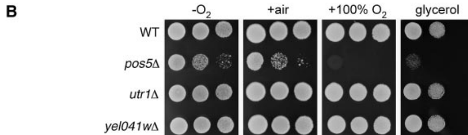
Fig. 3. Pos5p yeast homologs are not required for protection from hyperoxia or growth on a non-fermentable carbon source. (A) The amino acid sequences of S.cerevisiae Pos5p, Utr1p and Yel1041p and human PPNK (accession No. NP_075394) were aligned using Clustal_W 1.5. Identical residues are highlighted in black, and similar residues are outlined in gray. (B) The indicated strains were tested for growth as in Figures 1 and 2A. Strains utilized: wild-type, BY4741; pos5Δ , CO205; utr1Δ , BY4742 utr1Δ::kanMX4 ; yel1041wΔ , BY4741 yel1041wΔ::kanMX4 .
