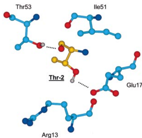
Fig. 4. Spatial orientation of residues in the SAP/SH2D1A SH2 domain (shown in cyan) involved in binding to the Thr-2 site (in gold) of the peptides. Protein residues shown are all within 4 Å of Thr-2 in both complexes. Oxygen atoms are colored red and nitrogen blue. Dashed lines indicate hydrogen-bonding interactions. Note that, except for the hydroxyls of the two Thr residues, hydrogen atoms are omitted for clarity.
