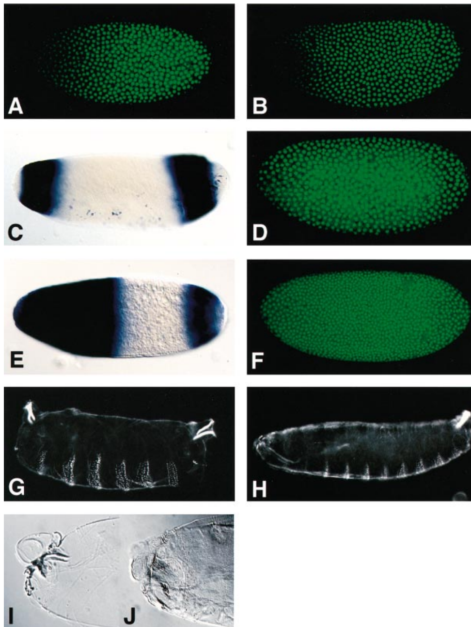
Fig. 3. Translational repression of cad mRNA in the anterior region of the embryo requires an intact PEST motif of Bcd. (A) Cad gradient formed in early Drosophila embryos (stage 11). (B) A transgene-expressed truncated version of Bcd ( Bcd^{1-202} , see Figure 2A) which removes several distinct C-terminal domains including most of the serine- and threonine-rich sequences required for transcriptional activation and causes a Cad gradient in embryos derived from bcd mutant females. Such embryos develop a bcd mutant phenotype (see cuticle preparation in G). (C) In situ hybridization showing that the posterior expression domain of hb is duplicated, whereas the anterior, Bcd-dependent expression domain of hb (see panel E for a wild-type-like expression pattern) is absent in such embryos. Thus, Bcd^{1-202} has lost the ability to activate transcription but maintains translational suppressor activity on cad mRNA. (D) Lack of Cad gradient formation in embryos derived from bcd mutant females expressing the Bcd^{1-185} transgene. (E–I) Alanine replacements within the C-terminal portion of the Bcd PEST motif interfere with translational repression of cad mRNA. In situ hybridization of an embryo from a bcd mutant female bearing the Bcd^{5ala} transgene (see Figure 2B and text) showing a wild-type like expression pattern of hb expression (E), indicating that Bcd^{5ala} causes activation of transcription. Anti-Cad antibody staining showing that Cad is present in the anterior region of a corresponding embryo (F). Thus, Bcd^{5ala} functions as a transcriptional activator but fails to suppress the translation of cad mRNA. However, it rescues the bcd mutant phenotype (G). Rescued embryos develop a normal larval segment pattern (H) associated with a severe but variable head defect (I) due to an aberrant head involution process (J). A corresponding head phenotype was observed when Cad was expressed throughout the embryo using the GAL4/UAS system (for details see text). Orientation of embryos is anterior to the left, dorsal side up. Cad protein distribution was monitored by fluorescent anti-Cad antibodies viewed by confocal microscopy (see Materials and methods).
