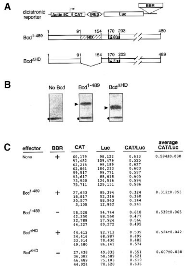
Fig. 1. Bcd-dependent regulation of translational repression in Drosophila Schneider cells. (A) Reporter gene designed to express a dicistronic transcript in which the cistrons chloramphenicol acetyltransferase (CAT) and luciferase (Luc) are separated by an internal ribosome entry site (IRES); the second cistron is followed by the SV40 3'UTR, including or excluding the BBR. The reporter genes are under the control of a constitutive promoter (actin 5C) and result in a dicistronic transcript. Translation of the 5' transcript (CAT) occurs in a cap-dependent manner, whereas translation of the 3' transcript (Luc) is IRES-dependent. Effector genes under the control of the actin 5C promoter express full-size Bcd (Bcd 1-489 ; sequence according to Berleth et al. , 1988) or an inactive Bcd (Bcd ΔHD ) in which the RNA-binding homeodomain (HD, position 91–154; hatched box) was deleted. (B) Western blots tested with polyclonal anti-Bcd antibodies, showing that the Bcd ΔHD control protein (see panel C) is produced in the cotransfected cells. Note the presence of a crossreacting band (dot) which served as an internal control for the amount of effector protein produced (arrowhead). (C) Translation-dependent reporter gene activities in cotransfected cells. 'None' refers to the absence of an effector gene; '+' or '-' BBR refers to the presence or absence of the BBR in the 3'UTR of the dicistronic mRNA. CAT and Luc activities are shown from eight independent transfection experiments involving new plasmid DNA preparations and batches of cultured cells. Note that the CAT activities and the ratio of CAT/Luc activities were altered by full-size Bcd (Bcd 1-489 ) when co-expressed with the BBR-containing reporter construct. Thus, Bcd 1-489 interferes primarily with cap-dependent translation of CAT. Mean values and standard deviations (±) are shown.
