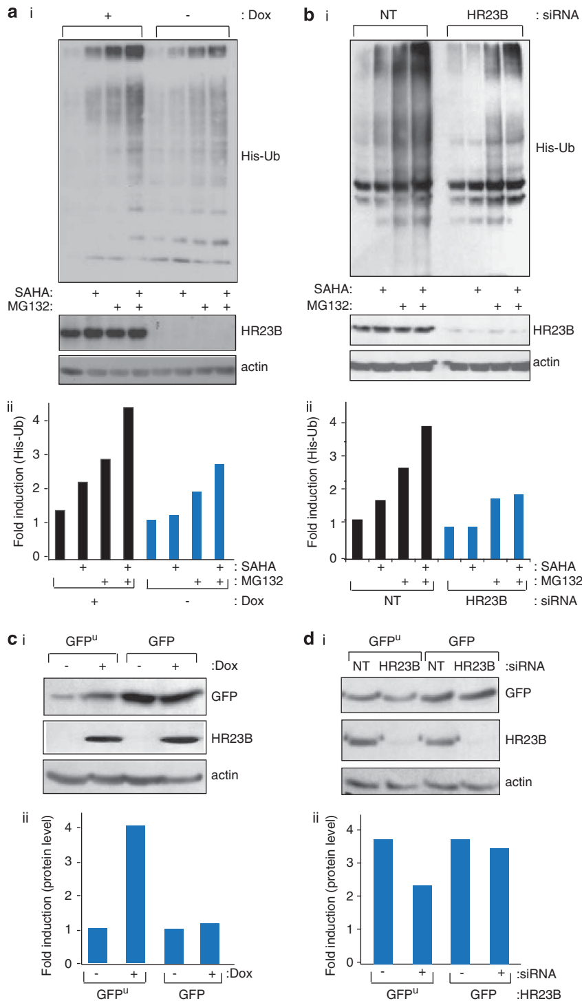
Figure 2 HR23B has an impact on the ubiquitin proteasome system. (a) (i) U2OS cells stably expressing inducible ectopic Flag-HR23B were transfected with His 6 -ubiquitin (His-Ub; 2 μg), then treated with doxycycline (+ and -, 1 μg/ml) for 24 h following an additional 20 h treatment with SAHA (5 μM) and/or 4 h treatment with MG132 (20 μM) as indicated. Cell lysates and Ni 2+ pull-down eluates were analysed by immunoblotting with anti-His as described. The input HR23B is shown underneath, together with actin levels. (ii) Quantitation of the ubiquitin signal. (b) (i) U2OS cells were transfected with control (NT) or HR23B siRNA (50 nM) for 24 h, then transiently transfected with His 6 -ubiquitin (His-Ub; 2 μg) for 24 h, following an additional 20 h treatment with SAHA (5 μM) and/or 4 h treatment with MG132 (20 μM) as indicated. Ni 2+ pull-down eluates were analysed by immunoblotting with anti-His. The input HR23B level is shown underneath, together with actin levels. (ii) Quantitation of the ubiquitin signal. (c) (i) U2OS cells expressing inducible ectopic Flag-HR23B were transiently transfected with GFP u or GFP (100 ng), then treated with or without doxycycline (+ or -, 1 μg/ml) for 24 h as indicated. Cell lysates were analysed as described. Levels of GFP, HR23B and actin are shown. (ii) Quantitation of the GFP signal. (d) (i) U2OS cells were transfected with control (NT) or HR23B siRNA (50 nM) for 24 h, then transiently transfected with GFP or GFP u (100 ng) for 48 h as indicated. Cell lysates were analysed as described above. Levels of GFP, HR23B and actin are shown. (ii) Quantitation of the GFP signal
