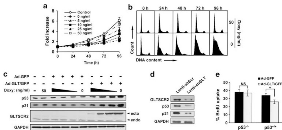
Figure 1 GLTSCR2 inhibits cell proliferation and cell cycle progression with p53 upregulation. (a) A549 cells were infected with Ad-GLT/GFP or Ad-GFP (control) with the indicated concentrations of doxycycline. Cell proliferation rates were assessed by counting cell numbers up to 96 h. The initial cell number was 1 \times 10^5 . Data are shown as the fold increase of three independent experiments (mean \pm S.D.). (b) The cell cycle profile analysis of cells infected by Ad-GLT/GFP for 4 days with the indicated concentration of doxycycline. (c) A549 cells were infected with Ad-GLT/GFP or Ad-GFP. After 24-h infection, cells were untreated or treated with decreasing amounts of doxycycline (50 ng/ml, 20 ng/ml, 10 ng/ml, and 0 ng/ml, respectively) for an additional 24 h. Cells were harvested and lysates were subjected to western blotting using the indicated antibodies (upper three panels) after normalization to GAPDH (lowermost panel); ecto, ectopic expression; endo, endogenous expression. (d) Knockdown of GLTSCR2 decreases the expression of p53 and downstream p21 protein. A549 cells were infected by GFP-tagged lentivirus targeting GLTSCR2 (Lenti-shGLT) or with scrambled (Lenti-shScr) shRNA. Lysates from Lenti-shGLT or Lenti-shScr cells were subjected to western blotting for evaluation of GLTSCR2 knockdown, or p53 and p21 expression, after normalization to GAPDH. (e) HCT116 ( p53^{+/+} ) and HCT116 ( p53^{-/-} ) cells were infected by Ad-GFP or Ad-GLT/GFP for 48 h and then pulsed with BrdU for 1 h before fixation. Cells with BrdU immunofluorescence were counted. Data represent percentage of cells with BrdU uptake (mean \pm S.D.) of three independent experiments. * P < 0.05 ; NS, not significant
