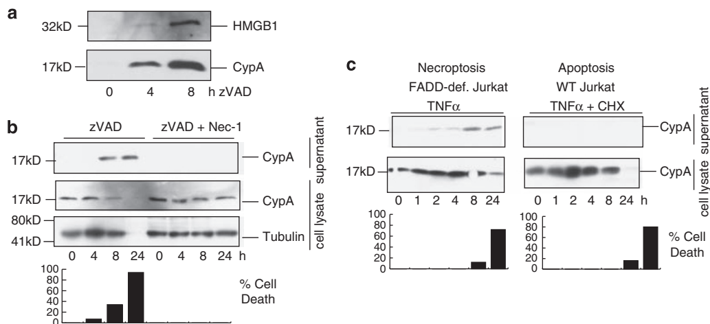
Figure 1 Cyclophilin A is released from necroptotic cells as a result of cytoplasmic membrane permeabilization. (a) L929 cells were treated with 100 \mu M zVAD.fmk for indicated hours. The supernatants were collected, concentrated and analyzed by SDS-PAGE followed by western blotting using anti-CypA and anti-HMGB1. (b) L929 cells were treated with 100 \mu M zVAD.fmk in the presence or absence of 30 \mu M Nec-1. The cell lysate and supernatant were analyzed by western blotting using anti-CypA. Anti-tubulin was used as a control. Cell viability was determined by ATP assay and indicated as a bar graph below. (c) FADD-deficient Jurkat cells (left panel) or wt Jurkat cells (right panel) were treated with 10 ng/ml hTNF \alpha to induce necroptosis, or 10 ng/ml hTNF \alpha + 0.5 \mu g/ml CHX to induce apoptosis, respectively. The cell lysate and supernatant were analyzed by western blotting using anti-CypA. The percentages of cell death were determined by ATP assay and indicated below
