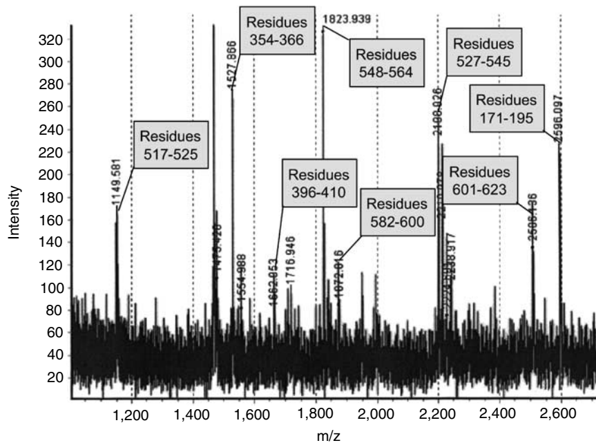
Figure 3 Peptide mass fingerprinting spectrum of mitofilin (mitochondrial inner membrane protein Q16891) obtained with an Ettan MALDI-ToF Pro as described in 'Materials and Methods'
