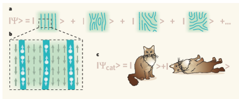
Figure 1 | Hunting the stripes. Electrons in the copper oxide planes of high-temperature superconductors sometimes form non-superconducting static stripe patterns. a , These stripes are believed to survive in the superconducting state as part of a quantum superposition of countless disordered stripe states that forms an overall featureless superconducting quantum liquid. b , Close up, the stripes are seen to consist of delocalized electrons ('rivers of charge') separated by domains of localized electrons showing a characteristic spin order. c , The principle of quantum superposition by which the stripe states are hidden from view in the superconducting phase is also the source of uncertainty over the fate of Schrödinger's infamous cat. Capturing the quantum cat or the quantum stripes in a definitive state requires snapshots taken on a timescale that is short compared with the timescale of quantum fluctuations between the superimposed states (dead or alive; stripy or non-stripy). By exploiting the coupling between high-frequency lattice and collective-stripe vibrations, Reznik et al. 1 provide a glimpse of quantum stripes.
