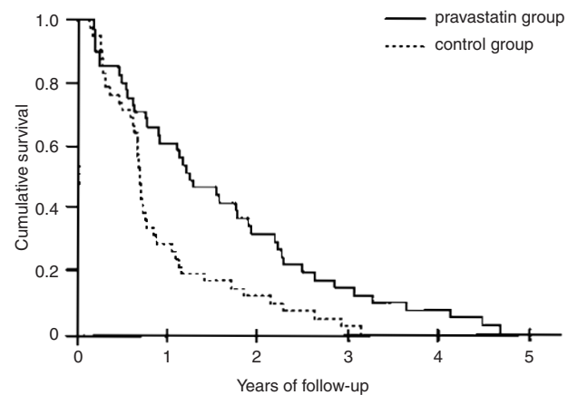
Figure 2 Kaplan-Meier survival curves in pravastatin ( n = 41 ) and control ( n = 42 ) groups. The median survival was 18 months in the pravastatin group and 9 months in the control group ( P = 0.006 by the log-rank test)
