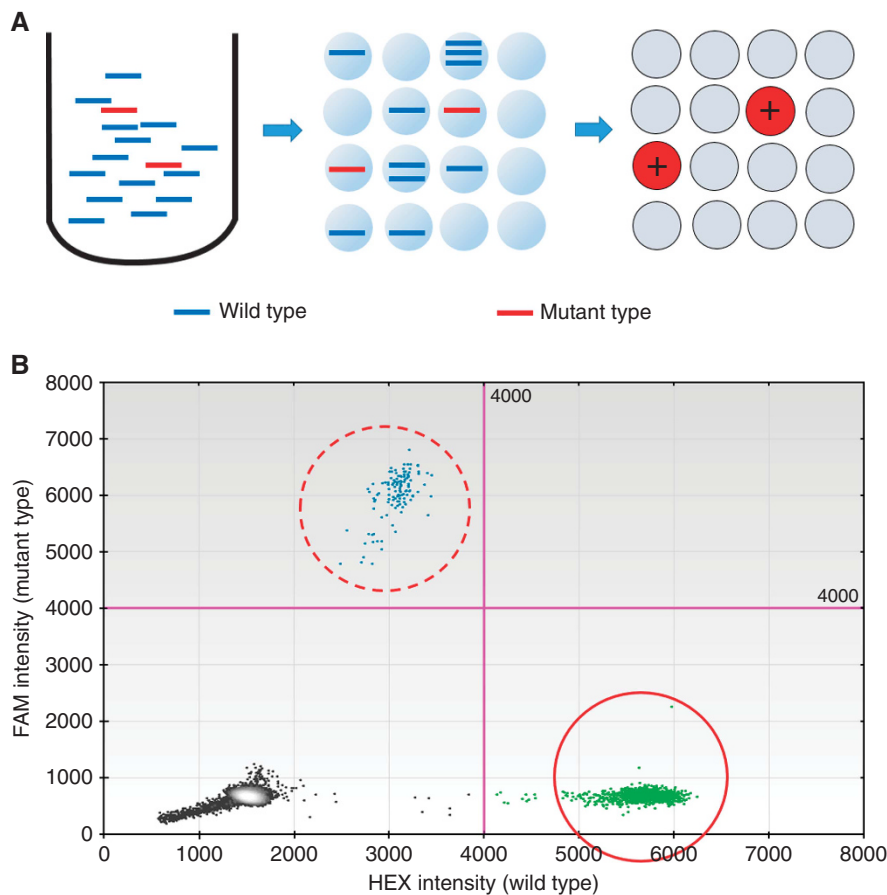
Figure 1. Overview of droplet digital PCR assay. (A) Schematic representation of the droplet digital PCR (ddPCR) assay, which is based on nanolitre-sized water-in-oil emulsion droplet technology. In this assay, target DNA molecules are uniformly distributed across thousands of emulsified droplets, after which PCR amplification is performed in each partitioned droplet. After amplification, reactions containing one or more target DNA molecules represent the positive end-point, whereas those without target DNA molecules represent the negative end-point. The number of target DNA molecules present can be calculated from the fraction of positive end-point reactions using Poisson statistics. (B) Two-dimensional histogram of ddPCR assay for KRAS amplification. FAM (blue) and HEX (green) fluorescence levels were plotted for each droplet. Clusters in the upper and right halves of the plot (dashed circle and solid circle) represent the positive mutant and wild-type KRAS end-point results, respectively.
