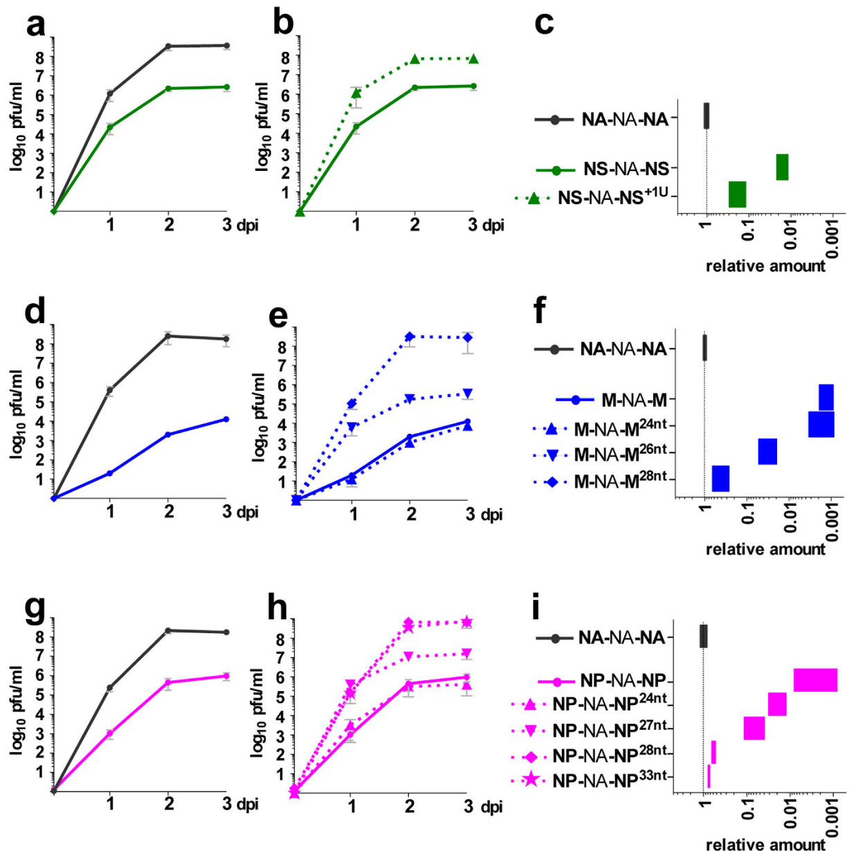
Figure 4. Effects on virus fitness and segment 6 incorporation of mutations acquired by X-NA-X viruses with a shorter 5'NC region. Panels (a–c), (d–f) and (g–i) correspond to NS-NA-NS, M-NA-M and NP-NA-NP viruses and mutants, respectively. (a, b, d, e, g and h) Growth kinetics. Infections were performed in MDCK cells at a low m.o.i. ( 10^{-5} pfu/cell). Titres were determined by standard plaque assays at indicated time points. Results correspond to the mean of at least two independent experiments. (c, f and i) Incorporation of segment 6. Viral RNAs were extracted from the supernatants collected at three days post infection of the growth kinetics and the NA segment vRNA level was evaluated by specific two-step RT-qPCR 19 . Results were expressed as relative amounts calculated using the 2^{-\Delta\Delta C_t} method with NA-NA-NA as virus reference and segment M as segment reference. Each bar represents the range (minimum - maximum) of the values obtained from the growth kinetics. Symbols used in growth kinetics graphs are presented next to the name of each virus in panels c, f and i.
