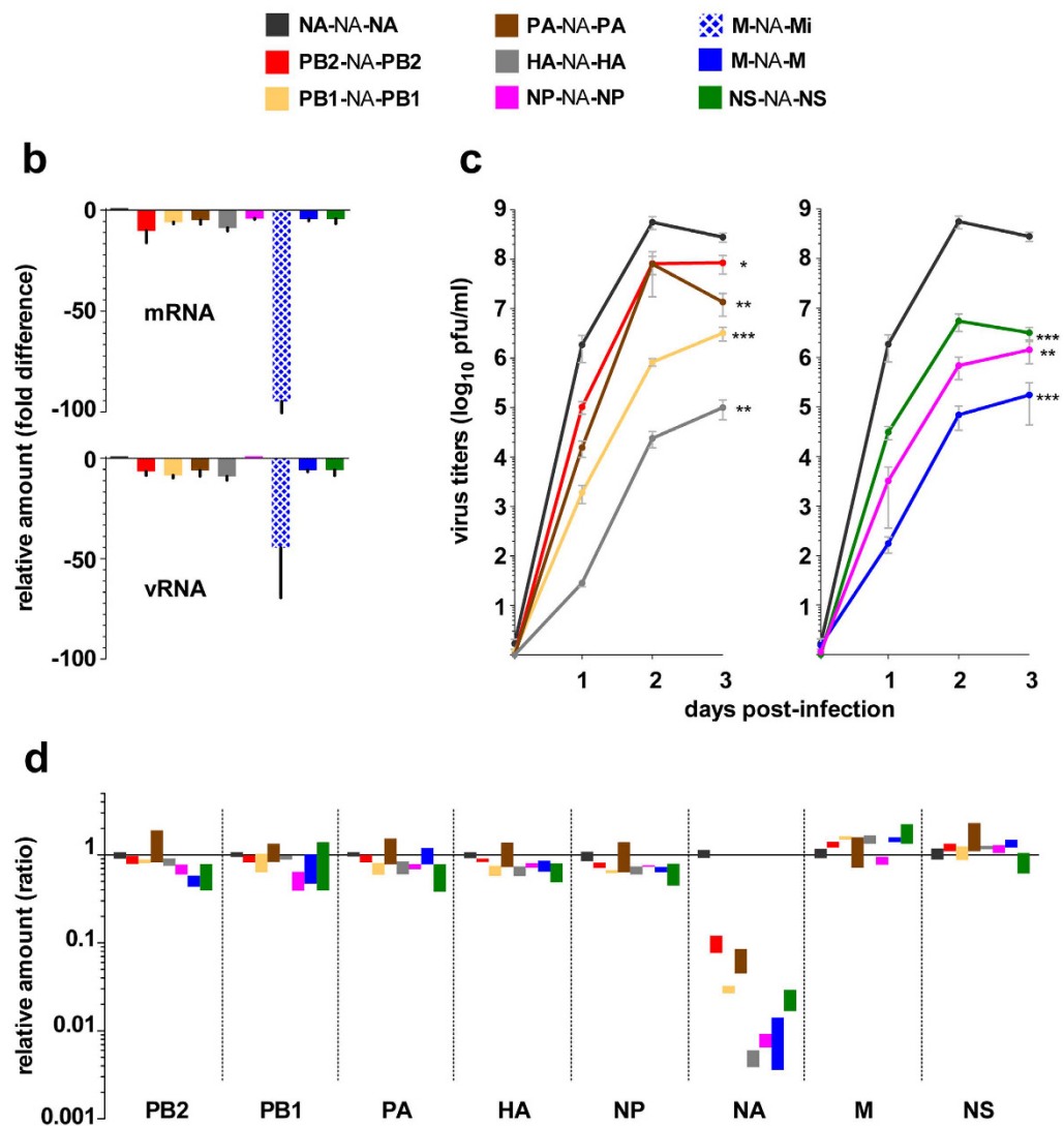
Figure 1. Effects of the replacement of the NA segment NC regions on transcription/replication, growth kinetics and segment incorporation. (a) Length, in nucleotides, of the WSN influenza virus 3' and 5' NC sequences of each segment (start and stop codons not included). Recombinant X-NA-X reverse genetics plasmids were constructed and each construct was assigned a colour code. (b) Transcription/replication of the X-NA-X genomic segments evaluated by transient reconstitution of functional vRNPs. 293 T cells were transfected and total RNA was extracted at 24 h post-transfection. The amounts of viral vRNA and mRNA were measured by specific two-step RT-qPCRs 19 . Fold differences relative to NA-NA-NA were calculated. Three independent experiments were performed and the mean (with Standard Error to the Mean, SEM) is given. (c) Growth kinetics of rescued X-NA-X viruses. Infections were performed in MDCK cells at a low m.o.i. ( 10^{-5} pfu/cell). Titres were determined by standard plaque assays at the indicated time points. Results correspond to the mean ( \pm SEM) of three independent experiments. Area Under Curve values were compared by t-test with NA-NA-NA as reference ( ^*0.05 < p\text{-value} < 0.01 ; ^{**}0.01 < p\text{-value} < 0.001 ; ^{***}p\text{-value} < 0.001 ). (d) Quantification of vRNA levels of the X-NA-X viruses. Viral RNAs were extracted from the supernatants collected at day three post infection of the growth kinetics in c and the level of each segment was evaluated by specific two-step RT-qPCR 19 . Results were expressed as relative amounts calculated using the 2^{-\Delta\Delta C_t} method with NA-NA-NA as virus reference and segment M as segment reference, except for segment M quantification where segment NP was used as segment reference. Each bar represents the range (minimum - maximum) of the values obtained from three independent growth kinetics.
