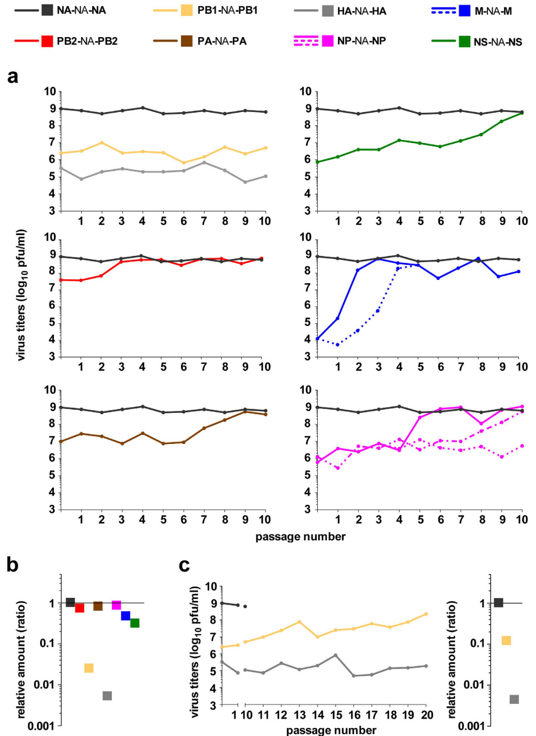
Figure 2. Effects of X-NA-X virus serial passages on virus fitness and segment 6 incorporation. (a) X-NA-X viruses were passaged in MDCK cells at a controlled low m.o.i. ( 10^{-5} pfu/cell). For each passage, supernatants were collected at day three post-infection, and virus titres were determined. Ten serial passages were performed for each virus. For M-NA-M and NP-NA-NP, one or two additional independent serial passages were performed, respectively. (b) Incorporation of segment 6 at passage 10. The NA segment vRNA level was evaluated by specific two-step RT-qPCR 19 . Results were expressed as relative amounts calculated using the 2^{-\Delta\Delta Ct} method with NA-NA-NA as virus reference and segment M as segment reference. (c) For the HA-NA-HA and PB1-NA-PB1 viruses, ten additional passages were performed and virus titres determined as in a (left panel). The level of segment 6 incorporation was evaluated at passage 20 as described in b (right panel).
