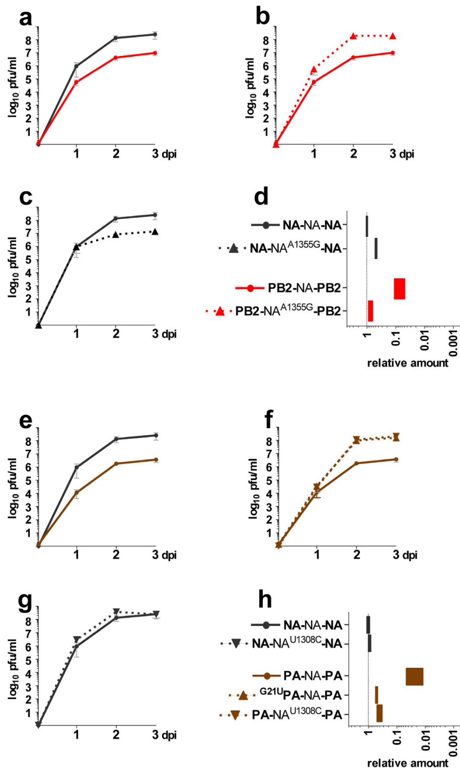
Figure 3. Effects on virus fitness and segment 6 incorporation of mutations acquired by X-NA-X viruses with a longer 5'NC region. Panels (a–d) and (e–h) correspond to PB2-NA-PB2 and PA-NA-PA viruses and mutants, respectively. (a–c and e–g) Growth kinetics. Infections were performed in MDCK cells at a low m.o.i. ( 10^{-5} pfu/cell). Titres were determined by standard plaque assays at indicated time points. Results correspond to the mean of at least two independent experiments. (d and h) Incorporation of segment 6. Viral RNAs were extracted from the supernatants collected at three days post infection of the growth kinetics and the NA segment vRNA level was evaluated by specific two-step RT-qPCR 19 . Results were expressed as relative amounts calculated using the 2^{-\Delta\Delta C_t} method with NA-NA-NA as virus reference and segment M as segment reference. Each bar represents the range (minimum - maximum) of the values obtained from the growth kinetics. Symbols used in the growth kinetics graphs are presented next to the name of each virus in panels d and h.
