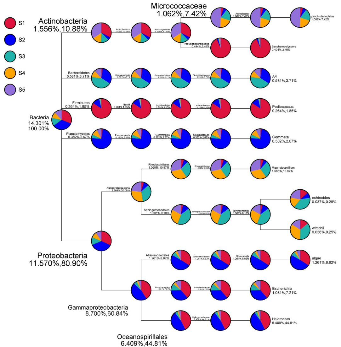
Figure 5. The relative abundance of each class based on 16S rDNA sequence analysis. The relative abundance is expressed in percentage and classification tree of complex samples. Different color of circle fan means different sample; the size of the fan means the relative abundance of proportional size on classification level of samples; The numbers below the classification name stand for the average percentage of relative abundance on this classification level in all samples. There were two numbers, the former one means the percentage of all species, the latter one means the percentage of selected species.
